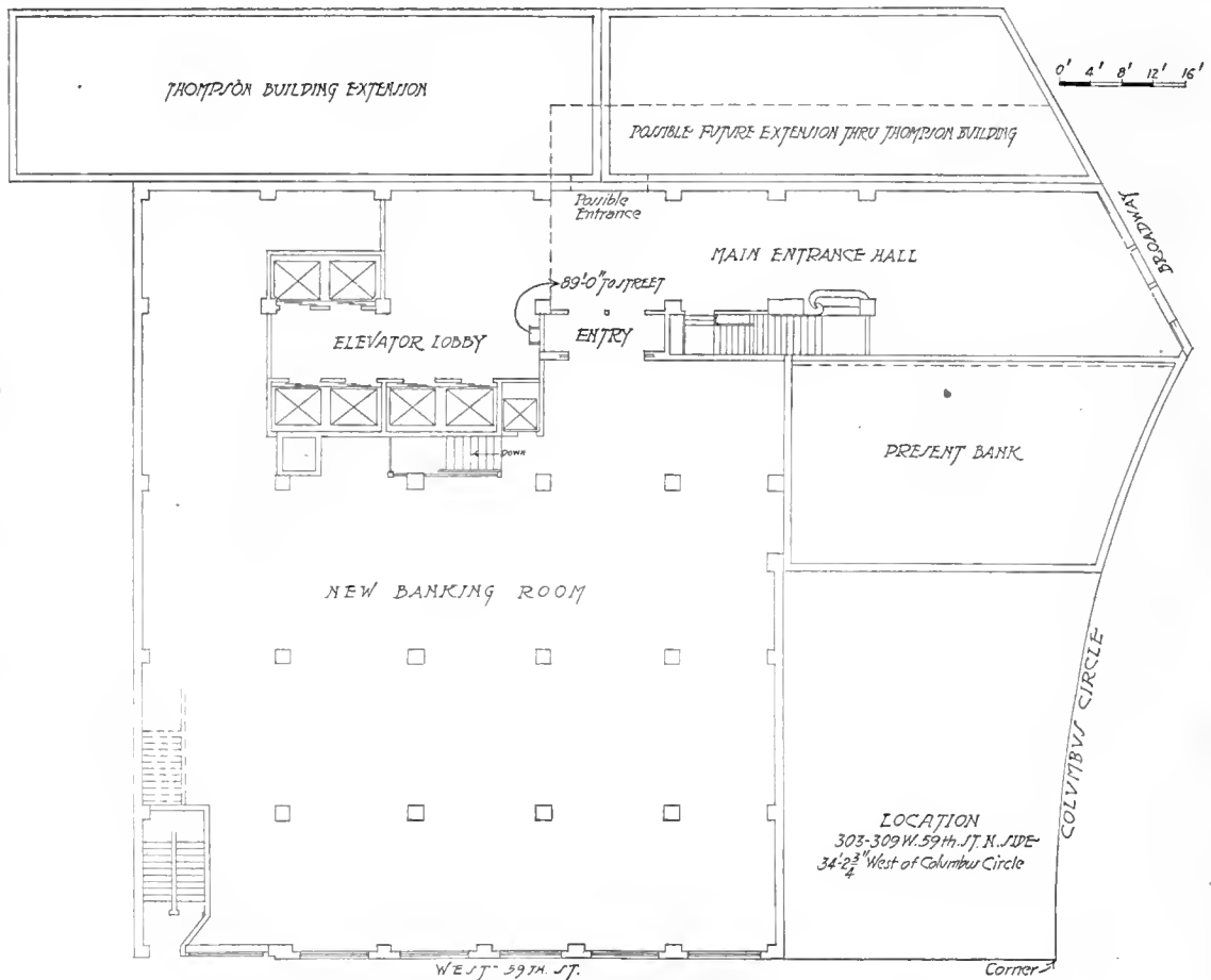
PLAN SHOWING LOCATION OF BUILDING ON SITE
